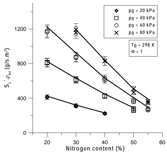
Figure 3: Laminar mass flow rate per unit area through the flame front in H 2 -N 2 O-N 2 mixtures as a function of nitrogen dilution and initial pressure. Kinetic model predictions are shown as solid lines.
