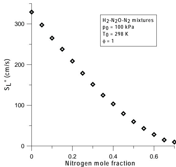
Figure 4: Laminar burning speeds calculated using the mechanism of Mueller et al. [33] for stoichiometric \text{H}_2\text{-N}_2\text{O-N}_2 mixtures with varying \text{N}_2 dilution.
